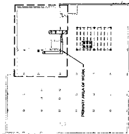
2 KEY PLAN G0-1 1/2" = 1'-0"
